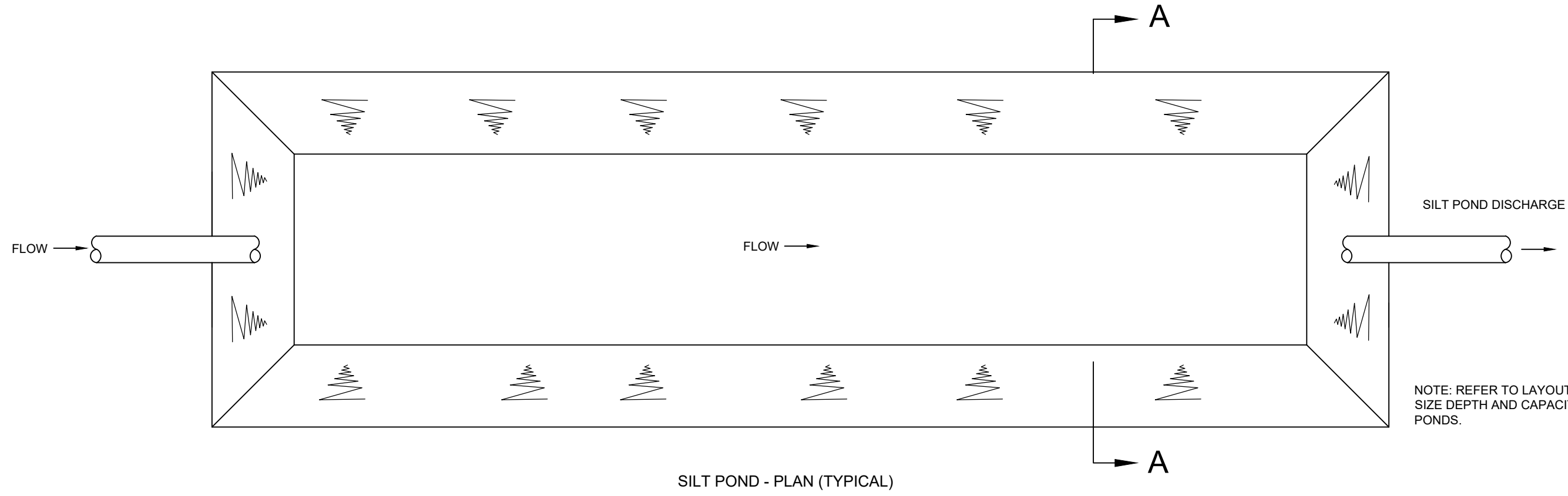
SILT POND - PLAN (TYPICAL)
